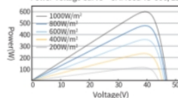
Power-Voltage Curve JAM66D45-600/LB
